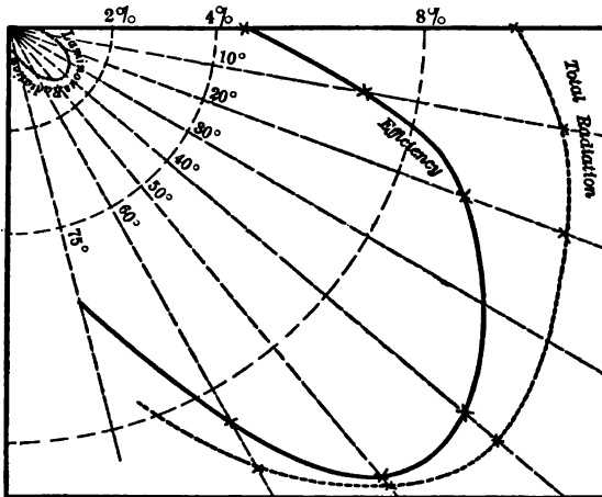
Fig. 1 Mean Hemi-Spherical Efficiency = 8.4%
